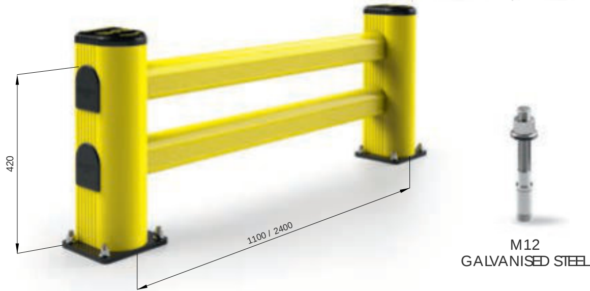
LM RACK END 1100x500 2400x500
