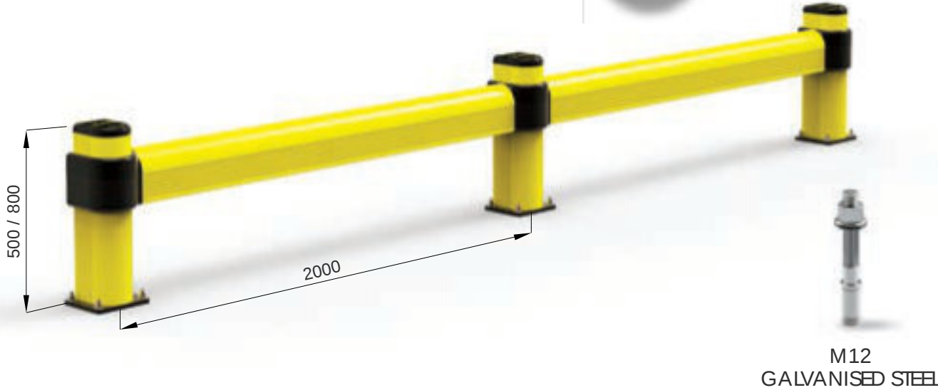
LINK SINGLE 500 800
