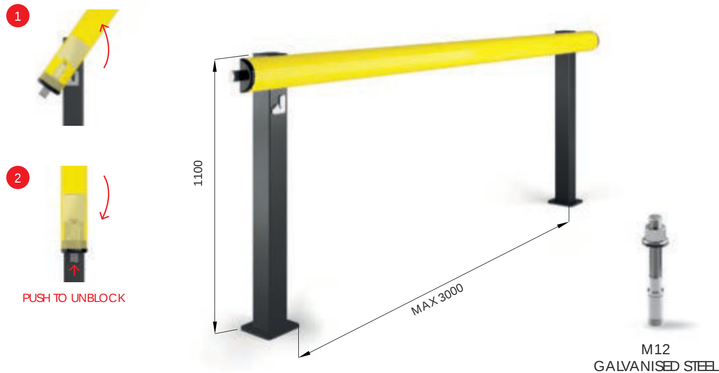
HUG GATE
