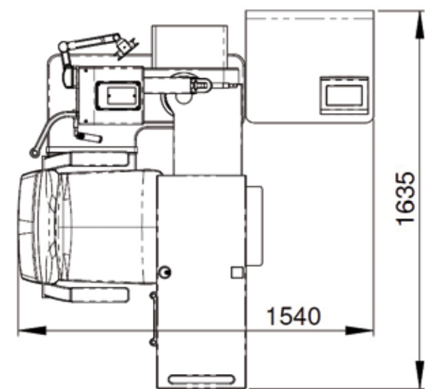
IS-1 footprint
