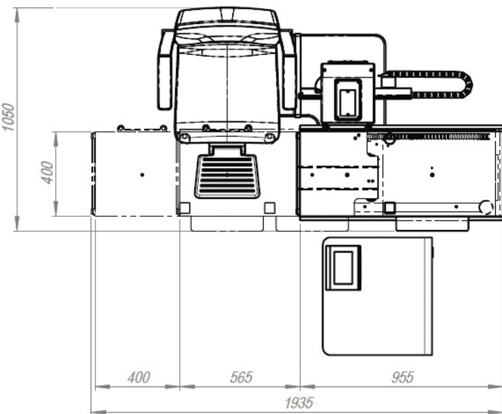
IS-1P footprint
