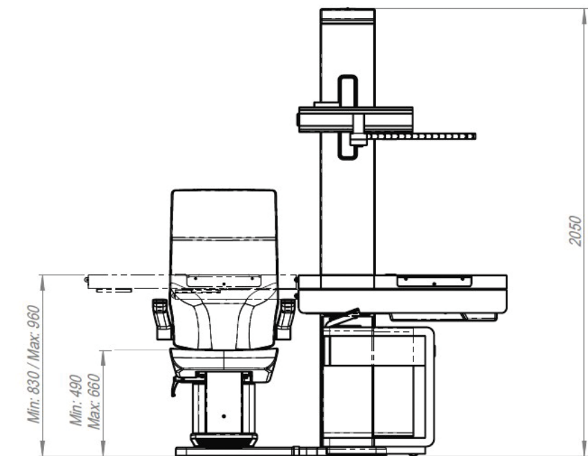
IS-1P dimensions
