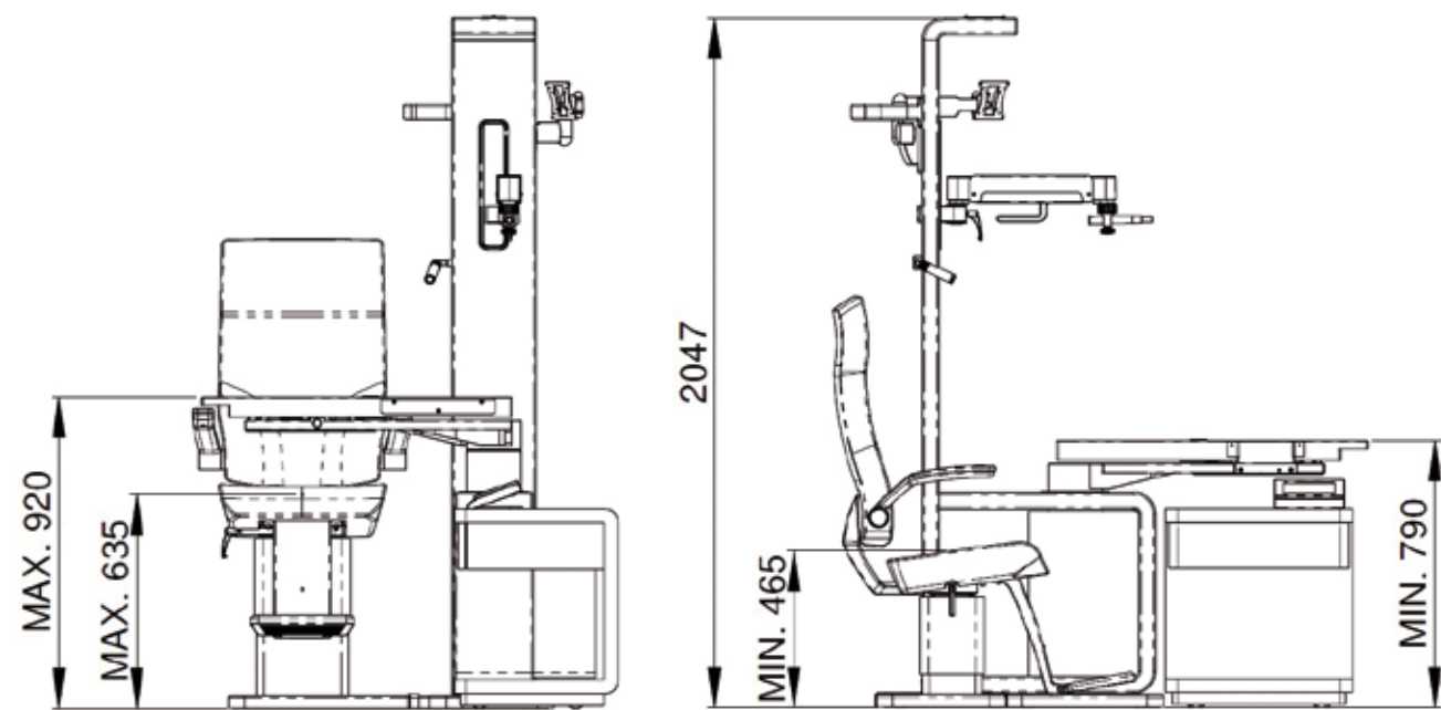
IS-1 & IS-1D dimensions
